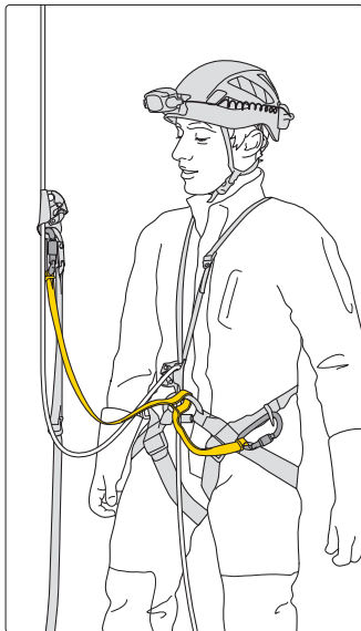
The asymmetrical SPELEGYCA double lanyard has multiple different uses when caving, such as tethering oneself, passing intermediate anchors, or ascending a rope.
