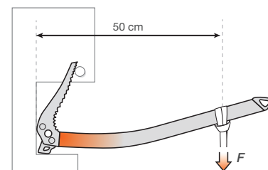
Shaft Insertion Strength Test
