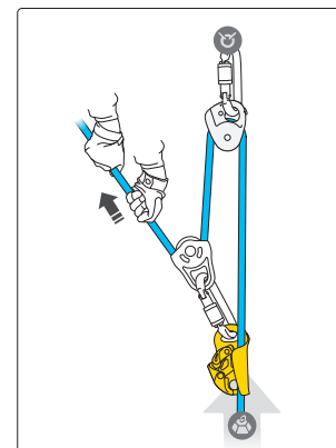
Pulley system with a BASIC ascender
