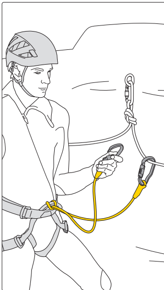
The DUAL CANYON CLUB, DUAL CANYON GUIDE, and DUAL CONNECT VARIO lanyards allow positioning at the anchor and progression along a lifeline when canyoning.
