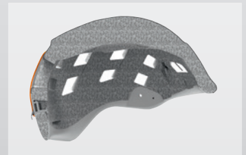
The low-profile design of the helmet is achieved using In-Mold construction with an expanded polystyrene (EPS) foam liner injected inside a lightweight polycarbonate shell.
