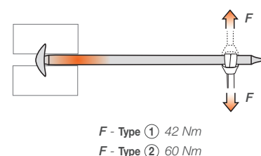
Levering Test
